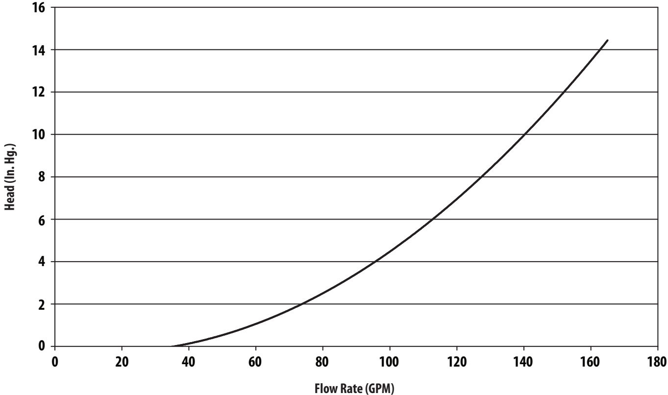
SPC-2 V Head Loss Curve
